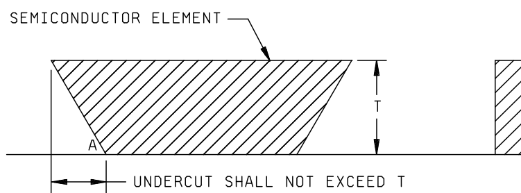
FIGURE 2012-6. Undercutting.
