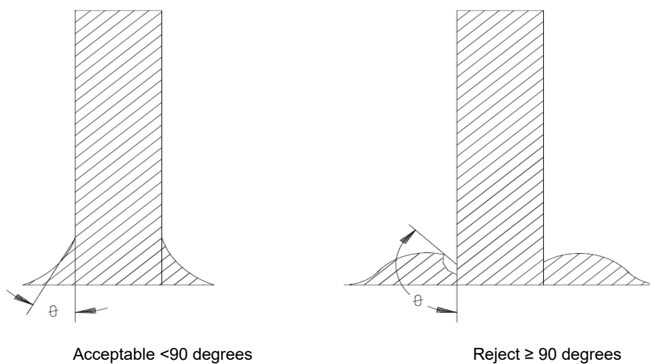
FIGURE 2003-11. Acceptable wetting angle for column grid arrays.
